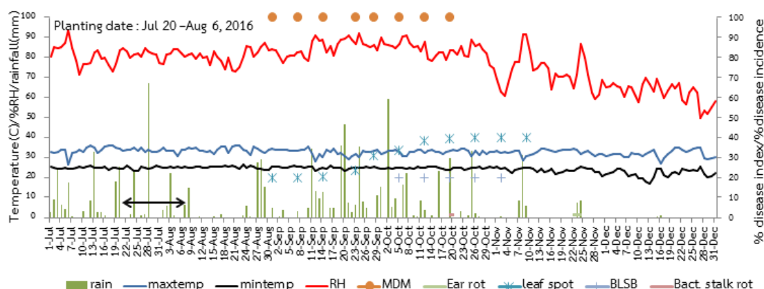
Figure 9 Meteorological data, average percent disease index and disease incidence of some diseases found on maize planted in late rainy season in 2016 at Nakhon Sawan. Arrow indicates range of planting date of surveyed fields. MDM=Maize dwarf mosaic, Leaf spot=Curvularia leaf spot, BLSB=Banded leaf and sheath blight, Bact. Stalk rot=Bacterial stalk rot.
