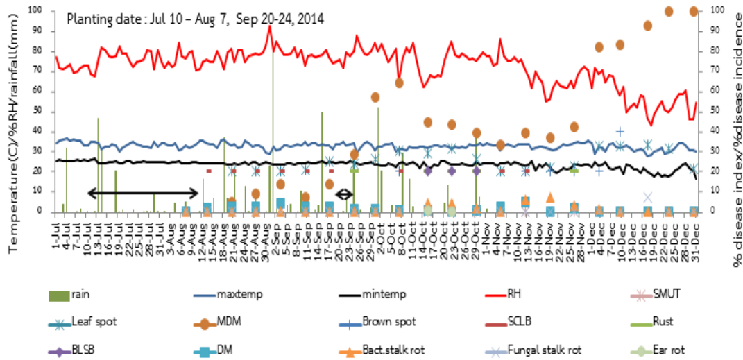
Figure 5 Meteorological data, average percent disease index and disease incidence of some diseases found on maize planted in late rainy season in 2014 at Nakhon Sawan. Arrow indicates range of planting date of surveyed fields. Leaf spot=Curvularia leaf spot, MDM=Maize dwarf mosaic, SCLB=Southern corn leaf blight, Rust=Southern rust, BLSB=Banded leaf and sheath blight, DM= Downy mildew, Bact. Stalk rot= Bacterial stalk rot.
