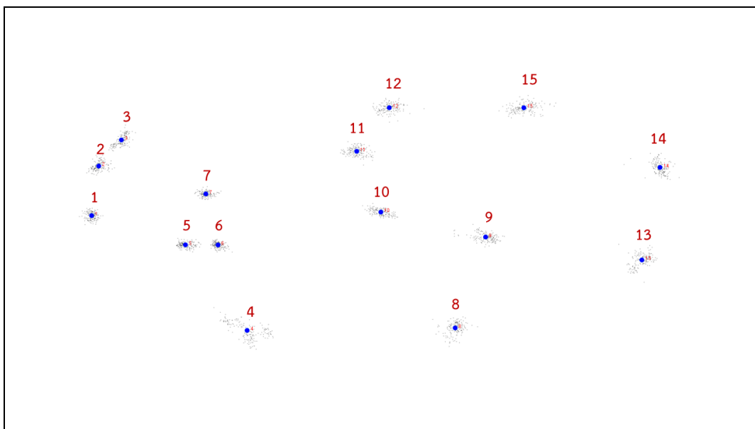
Figure 11 Procrustes superposition showing the variation of 15 landmarks of Dacini fruit fly wings from ten species. The figure shows the configurations of landmarks for which differences in position, scale and orientation have been removed. The position of the landmarks in relation to a real wing is shown in Figure 9.
