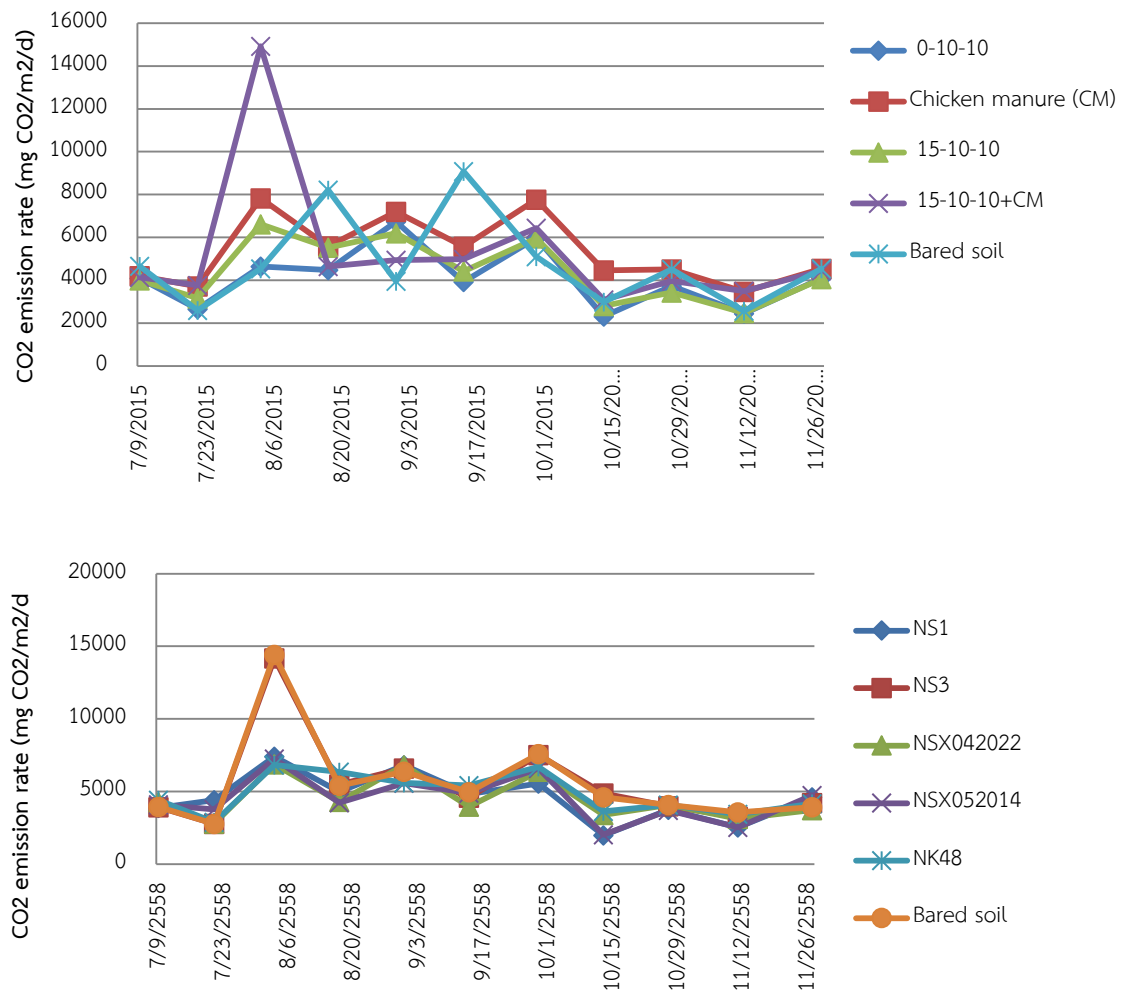
Figure 3 CO 2 emission from soil surface under different nitrogen fertilizer application of maize
