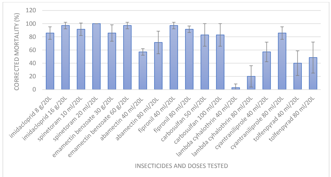
Figure 2 Mortality percentage ( \pm SD) of Scirtothrips dorsalis damaging chili from Wat Pleng district, Ratchaburi province, fed with chili leaves dipped with insecticides at recommended dose and two folds of recommended dose.
