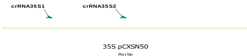
Figure 3. The crRNA position that serves as the cleavage site for the Cas12a (CPF1) enzyme
