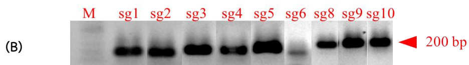
Figure 1 (A) CRISPR-Cas9 construct containing the sgRNA and (B) the sgRNA existence investigation using colony PCR technique with specific sgRNA forward primers and rgeb32-R 5'-GCCTTGACCCGAATTTGTGG-3
