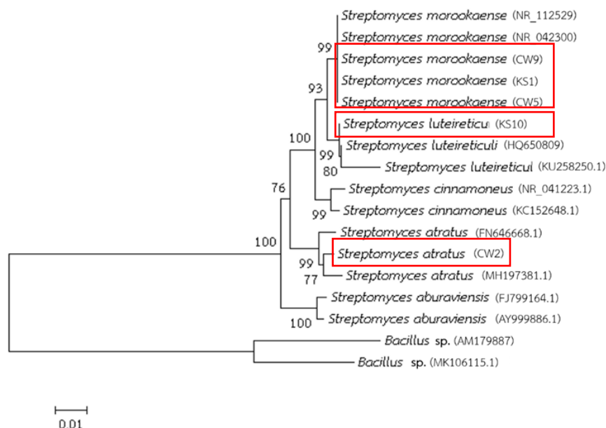
Figure 3 Phylogenetic relationships of the five Streptomyces strains based on 16S rRNA gene sequence analysis. The branching pattern was constructed by the neighbor-joining method. The number at each node refers to the bootstrap support value (%) based on 1000 replicates (greater than 50% are shown). The scale bar indicates 0.01 nucleotide substitutions per nucleotide position.
