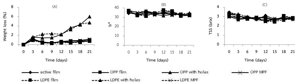
Figure 2 Change of weight loss (%) (A), b^* value (B) and TSS (brix) (C) of butterhead packed in different packaging during store at 5°C.
