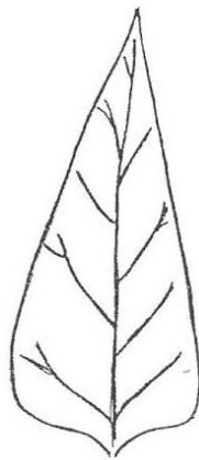
2 = Ovate-lanceolate
