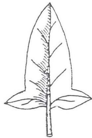
6 = Hastate
